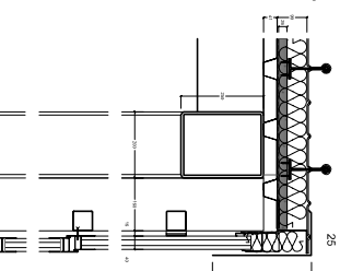
Detail 05
