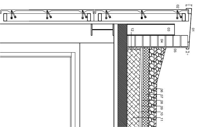
Detail 01
